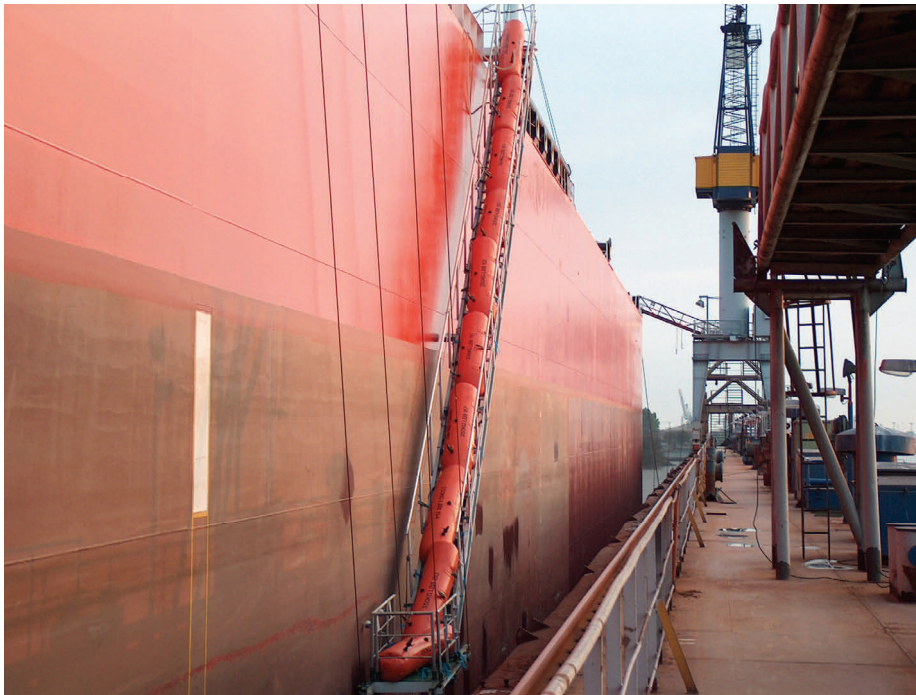
Accommodation ladder test at 3750kg
